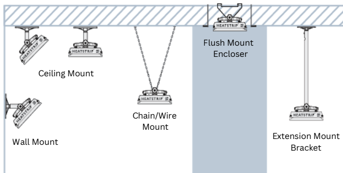
Optional ceiling-mount extension pole (Available in 4 lengths)
