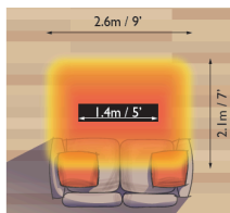
THH2400US-A Indoor direct overhead mounting
